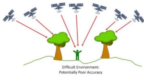
Fig. 11 Poor PDOP
